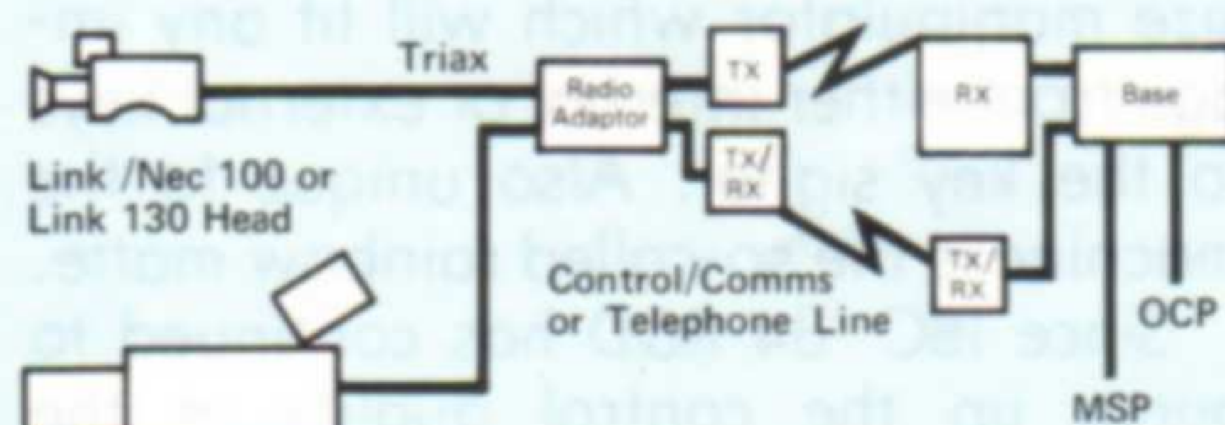
REMOTE OPERATION—UP TO 4 CAMERAS PER CONTROL LINK
