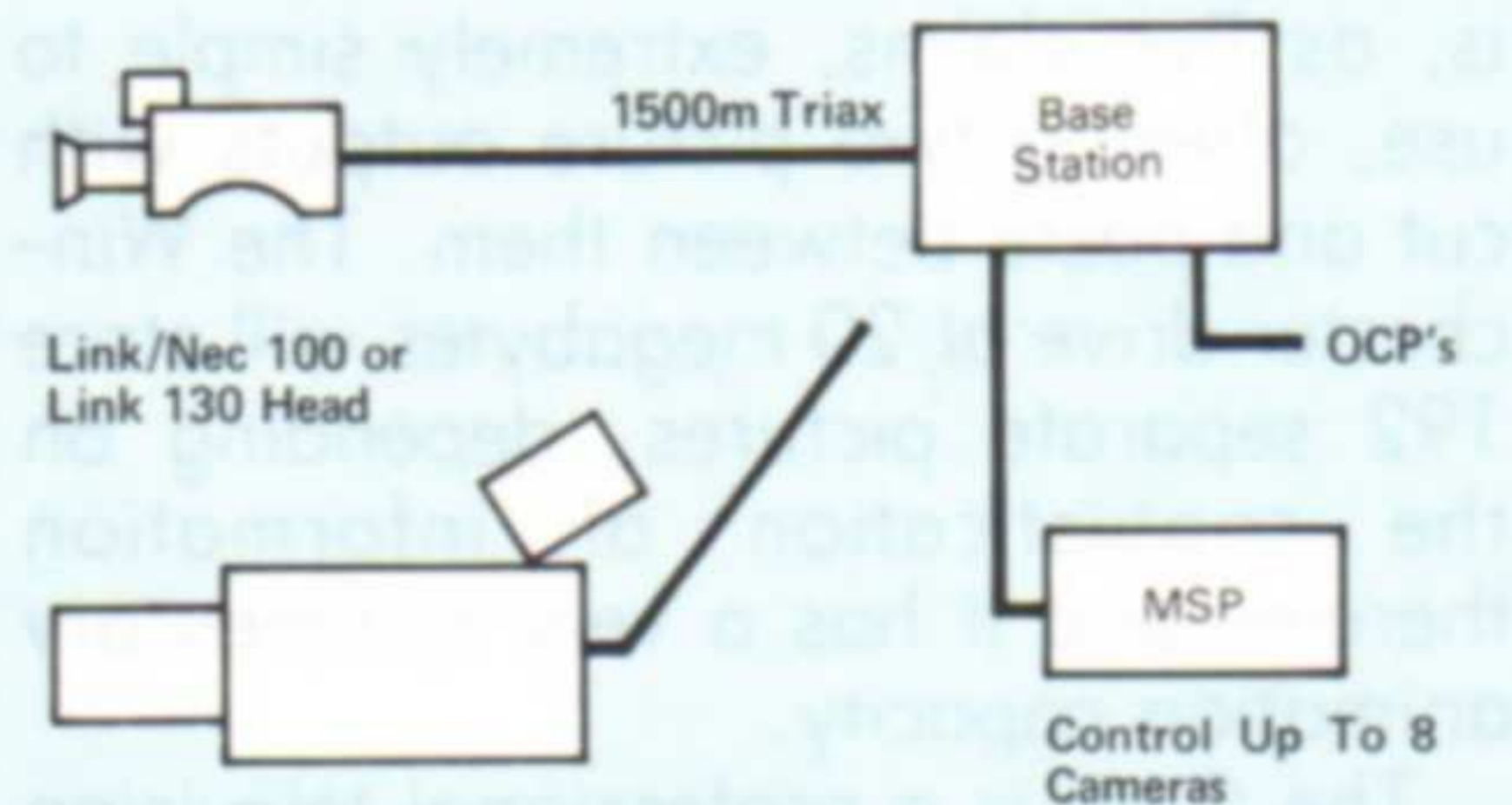
STANDARD TRIAX OPERATION
