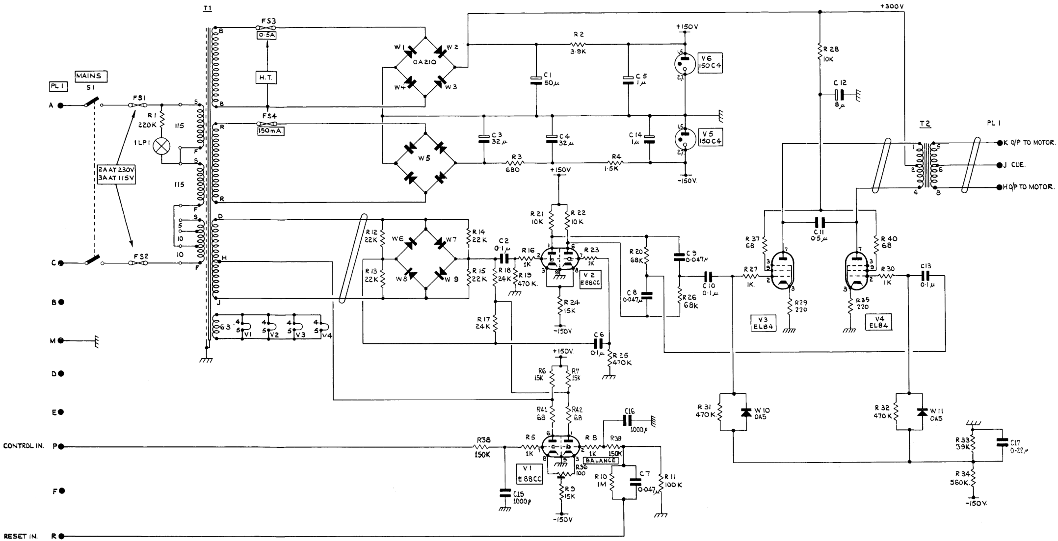
CAMERA CHANNEL 203 SERVO AMPLIFIER - CIRCUIT DIAGRAM
