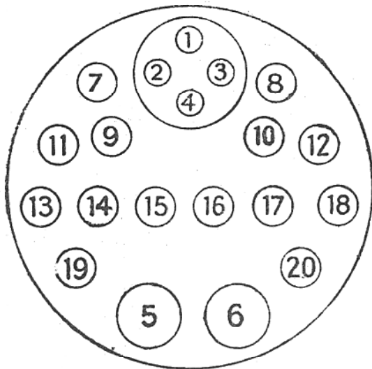
Figure 3. Plug
