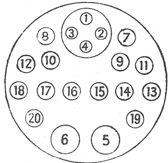
Figure 4. Socket
